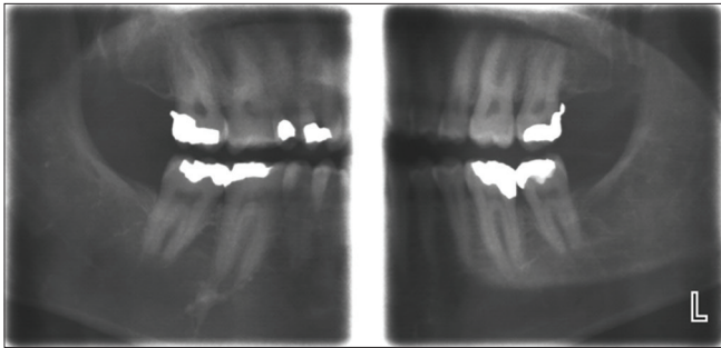
Figure 2: Bitewing radiograph of amalgam overhang for both teeth (No.2 and 17)
