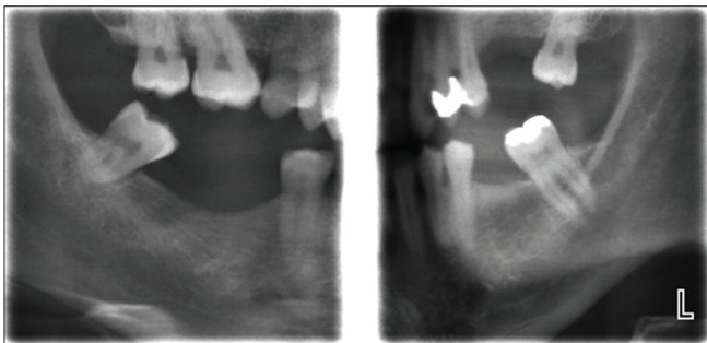
Figure 3: Bitewing radiograph of amalgam overhang for tooth (No.12)
