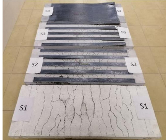
Figure 15. The crack patterns at bottom face of the specimens
