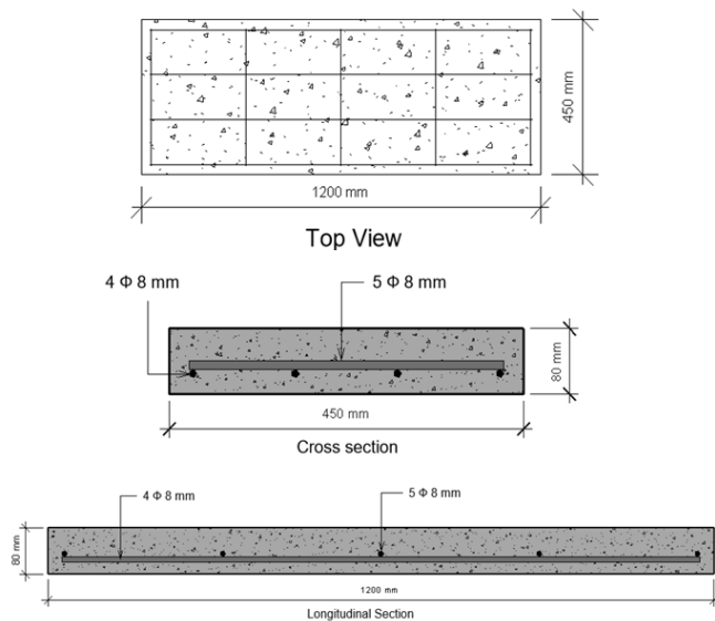
Figure 3. The details of one-way slabs
